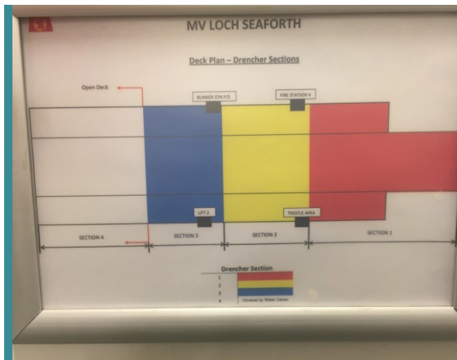
Fig 12: Colour coded car deck drencher sections
