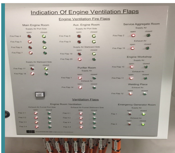
Fig 5: Remote ventilation flap indicators
