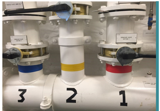
Fig 11: Drencher system valve labelling (colour coded)
