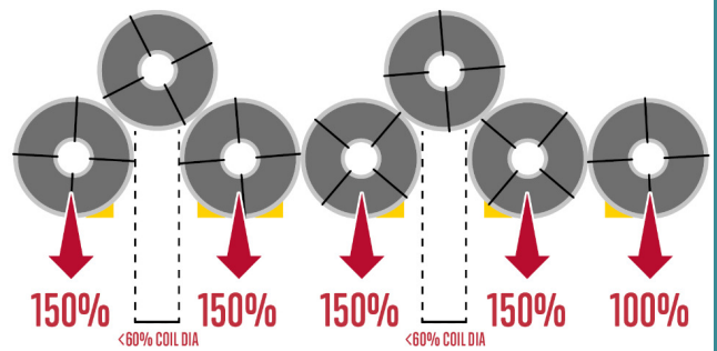
Double tier coils with locking coils.
