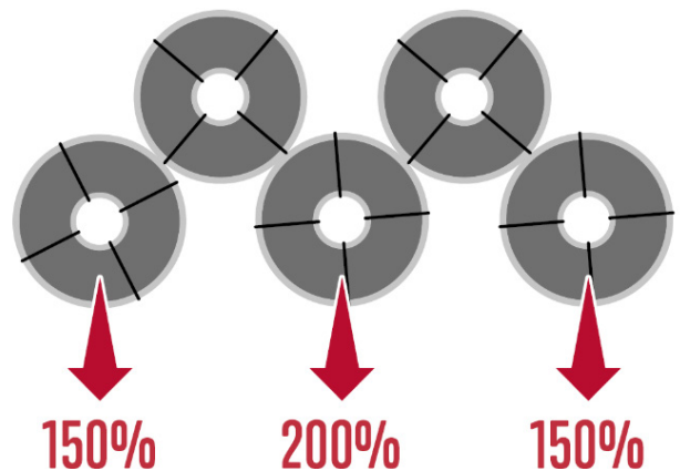
The load of the second tier coils transfers to the first further increasing the point load on the tank top.
