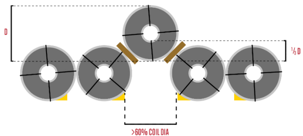
Locking coil with dunnage
