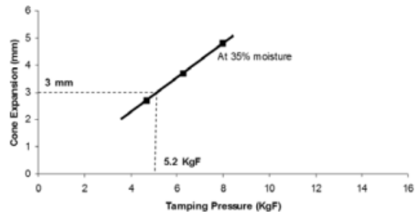
Figure 2. Effect of Tamping Pressure on Cone Expansion
